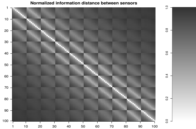
Figure 8: Normalized information distances between all pairs of sensors for the square visual field of 7(c) with 0 and 1 visualized as white and black, respectively. The distance between a sensor and itself is always zero, hence the white diagonal line. The further away two sensors are the less are they correlated and the greater is the information distance.
