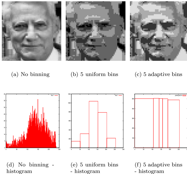
Figure 2: Figure 2(a) shows a 50 by 50 pixels grey-scale image of the founder of information theory, Claude Shannon, and figure 2(d) the corresponding histogram of pixels between 0 and 255. Figure 2(b) shows the same picture where the pixel data (0-255) is binned into only 5 different pixel values using uniform binning and figure 2(e) the frequency of pixel values. Finally, figure 2(c) shows the same picture with the pixel data binned into 5 bins using adaptive binning and figure 2(f) the corresponding histogram [ after (Olsson et al., 2005d)].
