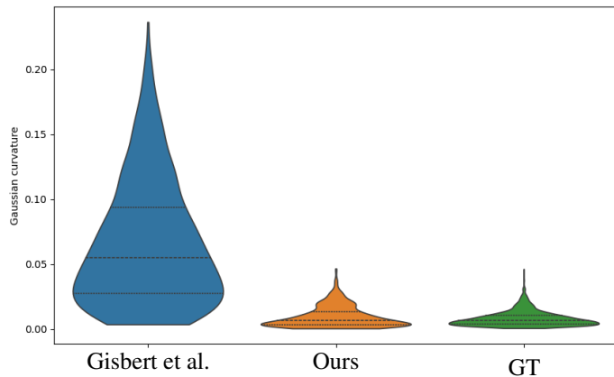
Fig. 9. Comparison of Gaussian curvatures respectively between the results produced by Gisbert et al. [11], our method and the ground truth. The measures were conducted on the test set of our ScarfFolds dataset.
