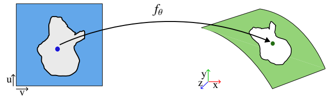
Fig. 5. Our trained network computes the neural 3D embedding of an entire patch of fabric to fill a partial 3D surface input (in green), after previously flattening it in 2D (in blue) using an isometric parametrization. For edition purposes, we can add additional constraints within the missing part.
