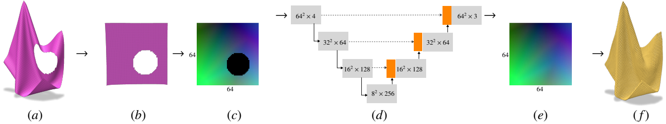
Fig. 2. Pipeline overview: starting from an input mesh with holes (a), we first parametrize the input geometry into a 2D domain (b) that is discretized into a 64 \times 64 4D image encoding the input mesh geometry (c) ( xyz -positions are encoded as RGB values) and a hole identifier mask. An attention U-net is used to inpaint the missing part (d, e) (convolution and downsampling blocks in grey, attention blocks in orange). A final point cloud can then be reconstructed (f).
