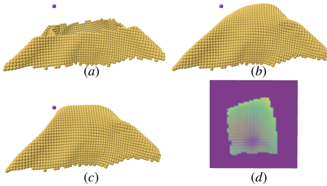
Fig. 7. The user sets a target point that for attracting the surface. The method automatically optimizes the best corresponding anchor point in the 2D parametric space and reconstructs the surface. From left-to-right, up-to-bottom: (a) Input; (b) First prediction; (c) Optimized surface, guided by the purple target; (d) Value and gradient of the anchor point adequacy in the parametric space.
