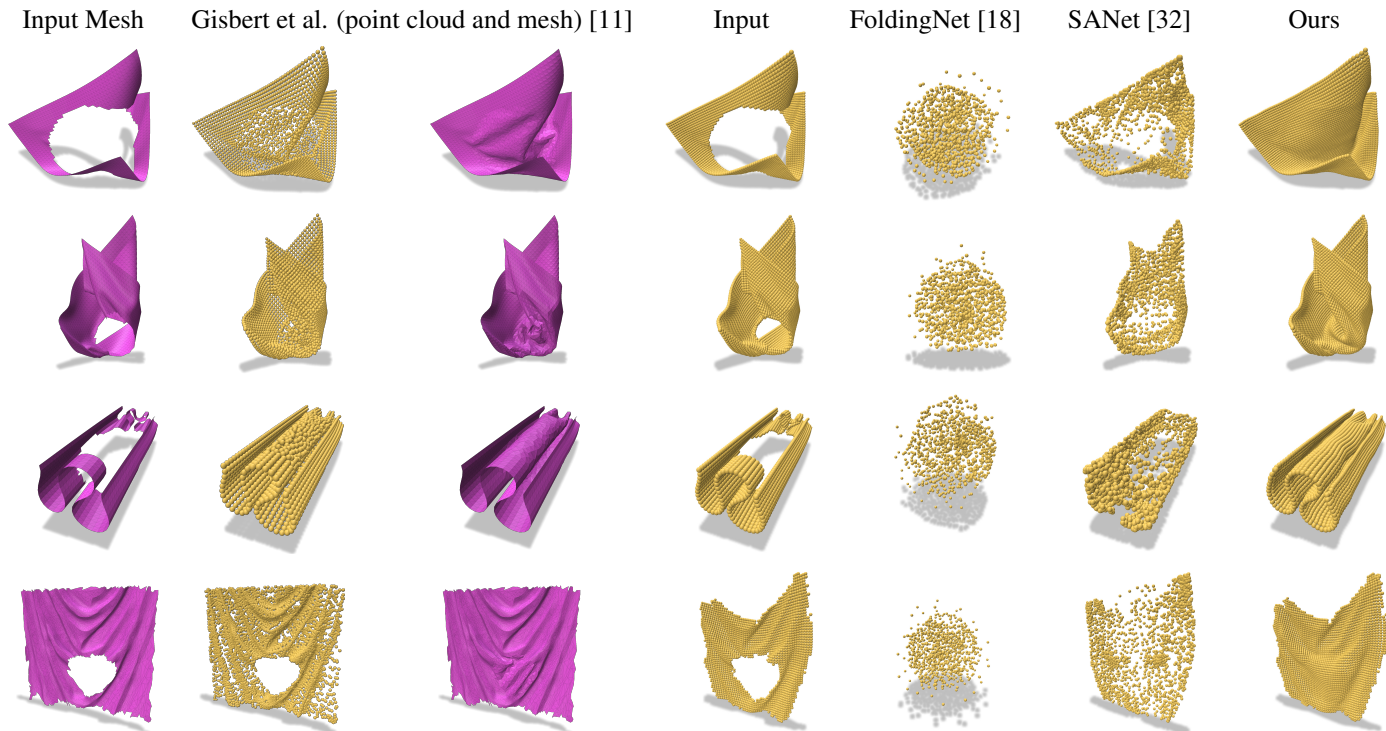
Fig. 8. Comparison between different hole filling methods. The two first rows are test examples from the dataset, the third one is a curtain obtained with a simulation, and the fourth row is taken from a statue scan (caryatid). The statistics regarding the 3D distance between neighbor grid points by using our neural approach is the following : mean: 0.01493, variance: 1.434e-06 (first row) mean: 0.01526, variance: 2.235e-06 (second row) mean: 0.01608, variance: 7.872e-07 (third row) mean: 0.01476, variance: 4.028e-06 (fourth row)
