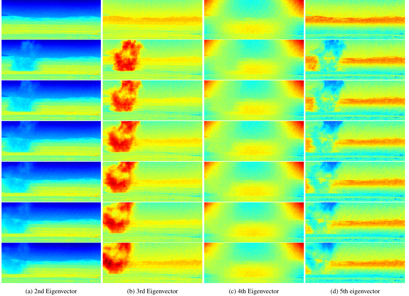
Fig. 1: Eigenvectors of the symmetric normalized graph Laplacian (1) for the 7 video frames shown in false color.
