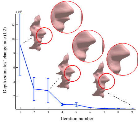
Figure 5. Convergence of the iterative optimization. The L2 distance between depth maps estimated in successive iterations, along with the Standard Errors, averaged over all 76 queries. Alongside the convergence, we provide an example reconstruction, demonstrating how features inconsistent with the appearance-shape of the reference face, gradually dissolve. Note that the first iteration is equivalent to depth estimation using SIFT-Flow alone ([17], see also Sec. 4.1).
