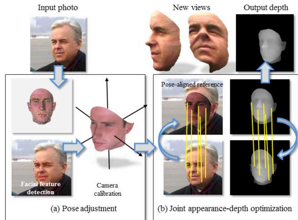
Figure 3. Overview of our depth estimation process. (a) During pose adjustment we obtain a camera matrix for the query photo, given detected facial features (Sec. 3.1). (b) Using this matrix, the reference, 3D model is re-rendered and our joint appearance-depth optimization process is applied using the aligned, rendered reference and its depth (Sec. 3.2). Note the reference photo superimposed on the query. See Sec. 3.2 for further details.
