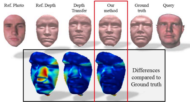
Figure 6. Visual comparison of different reconstruction methods. Shapes estimated for an example query in our empirical tests (Table 1). From left to right: The reference photo and depth-map; Depth-Transfer [13]; our own method; the ground truth depth; finally, the query photo. We provide also the \log_{10} absolute difference between the estimated and ground truth depth at each pixel, superimposed on the ground truth depth. Here, darker (bluer) colors are better – implying smaller differences.
