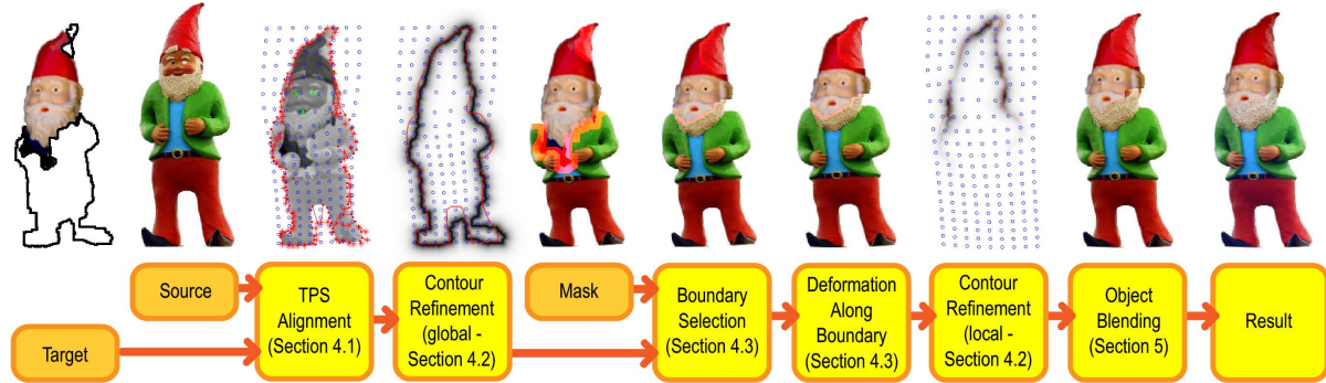
Figure 3: The alignment deformation pipeline is common to most of the demonstrated applications combining a pair of objects along a mask. The mask is either given explicitly or implicitly, depending on the application. In this pipeline, we first optimize a global deformation by TPS alignment via key-point correspondences. Then, we apply an exterior contour alignment to refine the deformation on the exterior boundary. Next, we calculate an optimized internal boundary to minimize the visual artifacts along the boundary between the two objects. Lastly, deformation and contour alignment is applied along this internal boundary to reduce the distortion and shape discontinuity.
