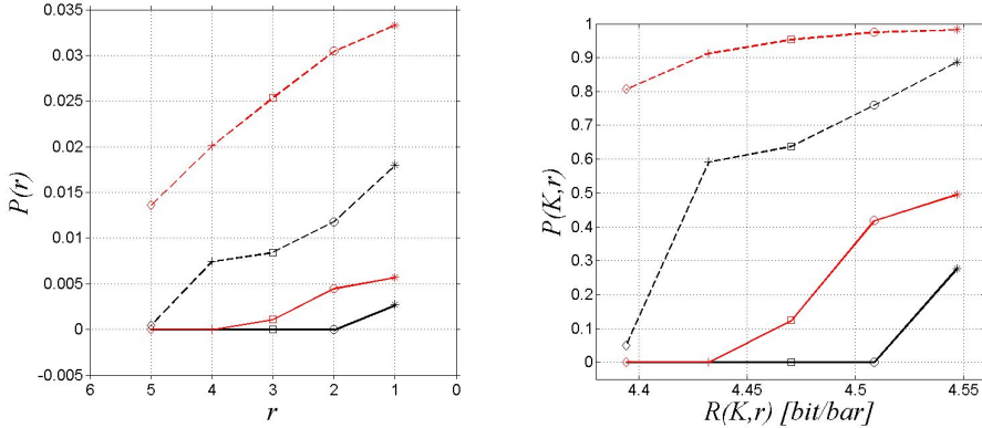
Fig. 5. Left: the probability of incorrect decoding P_E(r) to decode a single color patch as a function of the number of reference colors r . Right: the probability incorrect detection P_E(K,r) for a length K = 120 barcode versus the information rate compute using Eq. (1) and (2). ‘*’: r = 1 ; ‘o’: r = 2 ; ‘□’: r = 3 ; ‘+’: r = 4 ; ‘◇’: r = 5 . Subspaces learnt via PCA (solid line) over 32 illuminants, and diagonal model (dashed line). Black line: the algorithm tested on data with zero viewing angle. Red line: the algorithm tested on data with different viewing points ranging from -50 to 50 degrees.
