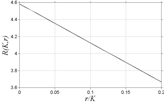
Fig. 1. The information rate for N = 24 , a length K = 120 barcode, and varying r from 0 to 24 reference colors
