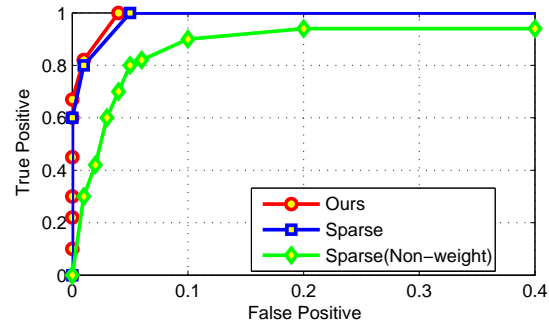
Figure 9. The detection results of UMN dataset.
