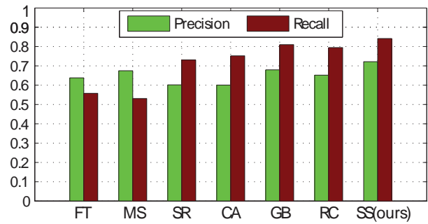
Figure 9. Automatic salient object segmentation.
