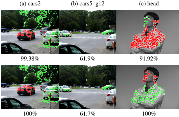
Figure 6: Segmentation results and the correctness ratios by the algorithm of Sugaya and Kanatani [20]. Above: original Hopkins155. Below: after incorrect trajectories have been removed. [20]
