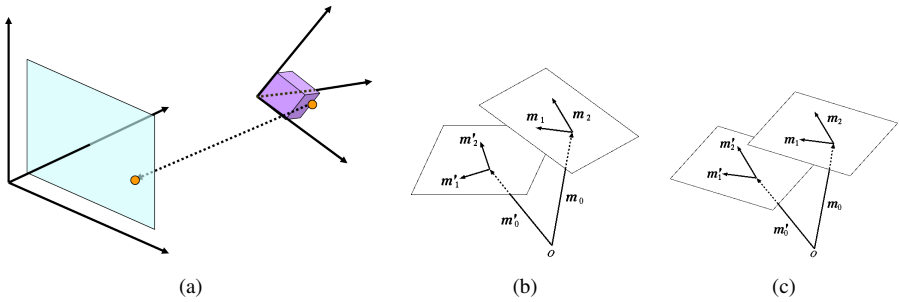
Figure 1: (a) Affine camera modeling. (b) The trajectories of points in in-plane motions are constrained to be in 2-D affine spaces. (c) The trajectories of translating points are constrained to be in parallel 2-D affine spaces.
