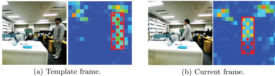
Fig. 3. Online template update. The red points in (a) indicate sampling points to make thermo-spatial sensitive histograms, and the orange points in (b) indicate the sampling points of the updated histograms that had stable similarities to the template. In this case, template histograms are updated only on histograms made from the orange points.
