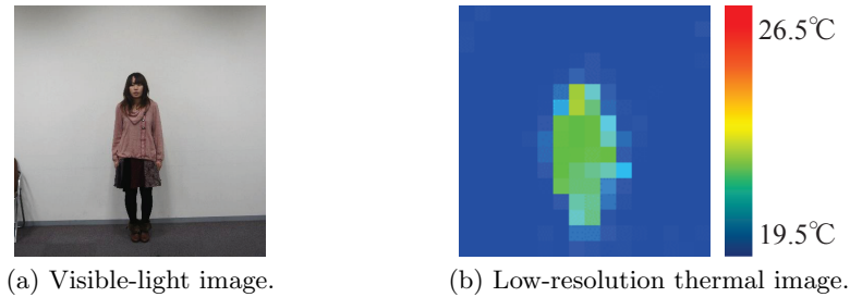
Fig. 1. Example of an output of a 16 \times 16 far-infrared sensor array. It is very difficult to identify the person from (b). Note that, this far-infrared sensor array outputs temperature lower than the actual body temperature. (a) is captured by a visible light camera put on the same position as the far-infrared sensor array.
