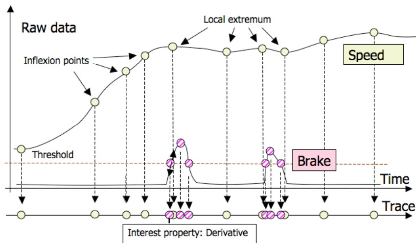
Figure 1. Discretization of analogical traces (Georgeon, 2008).
