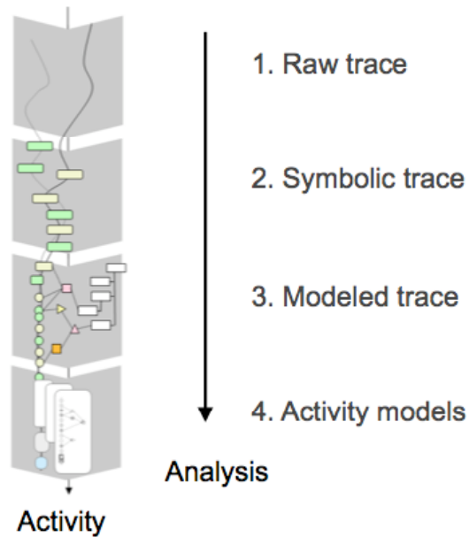
Figure 10: Activity modeling from activity traces
